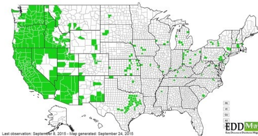
Centaurea solstitialis
